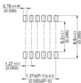
Leiterplatten - PCB - Layout (Top view)
